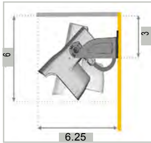
Wall mounting
