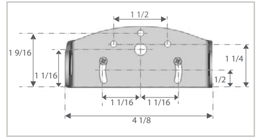
Bracket dimensions
